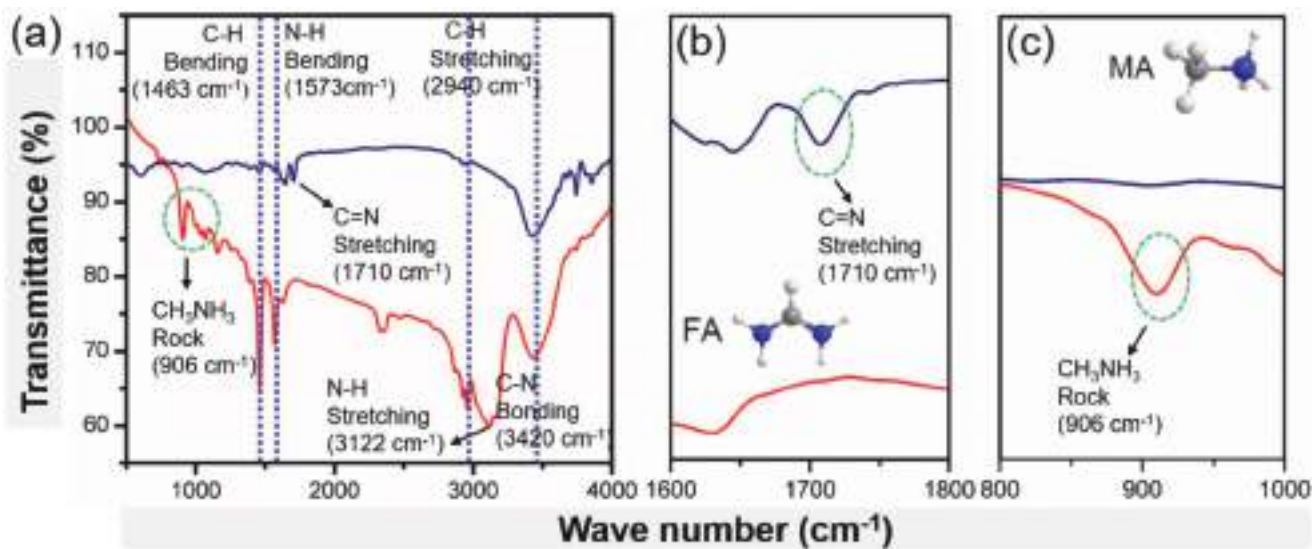
Figure 4. a) FT-IR spectra of fresh (\text{BA})_2\text{FAPb}_2\text{I}_7 (blue curve) and (\text{BA})_2\text{MAPb}_2\text{I}_7 (red curve) crystals in an open atmosphere. b,c) The formation of characteristics -\text{C}=\text{N} stretching band at 1710\text{ cm}^{-1} observed for the FA is absent in MA (b) and the band at 906\text{ cm}^{-1} corresponding to \text{CH}_3\text{NH}_3 rocking is absent for FA (c).
